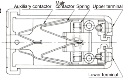
Diagram of contactor for current (KTT-AW□)
